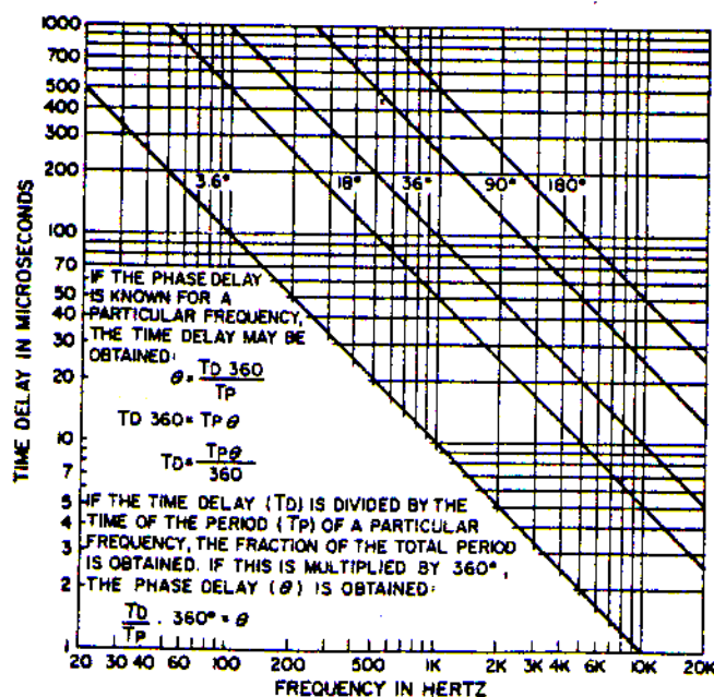
Fig. 5—Relationship of phase angle vs. frequency for constant time delays.
