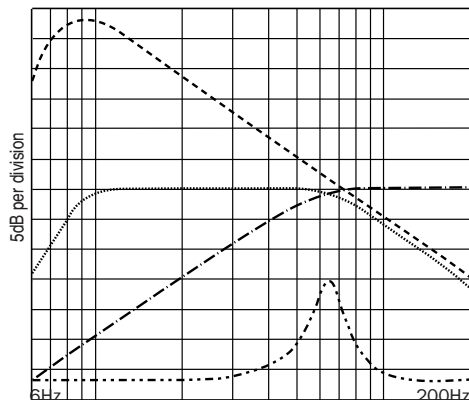
Electrical frequency response of the INFRAdual integrator Acoustical output of the INFRAsystem Acoustical frequency response of the INFRAloudspeaker in a sealed box Impedance amplitude of INFRAloudspeaker in a sealed box
